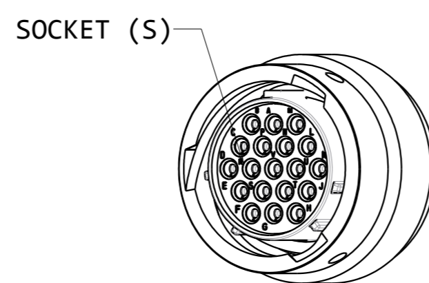
FEMALE CONNECTOR
