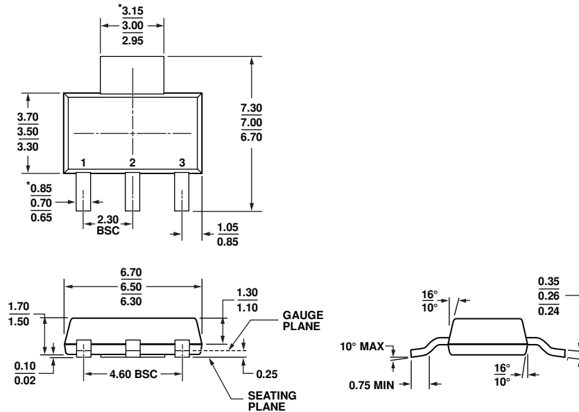
Figure 23. 3-Lead Small Outline Transistor Package [SOT-223] (KC-3)
