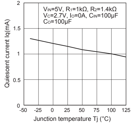
Fig.10 Quiescent Current vs. Junction Temperature
