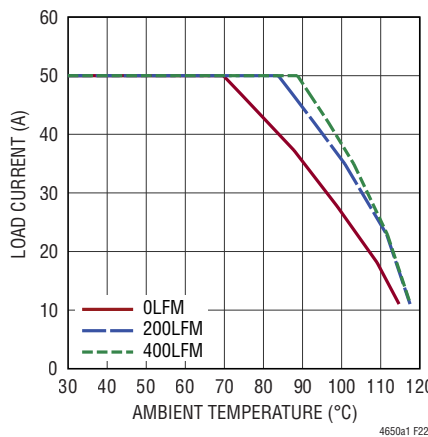
Figure 22. 5V to 1V Derating Curve, BGA Heat Sink
