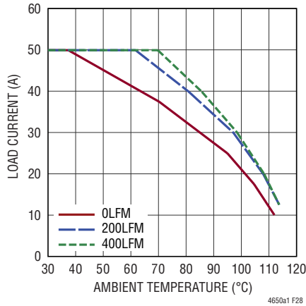
Figure 28. 5V to 3.3V Derating Curve, No Heat Sink
