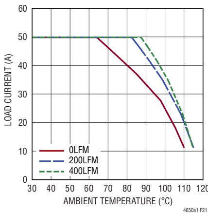
Figure 21. 12V to 1V Derating Curve, BGA Heat Sink
