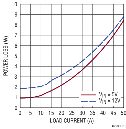
Figure 16. 1.8V OUT Power Loss Curve
