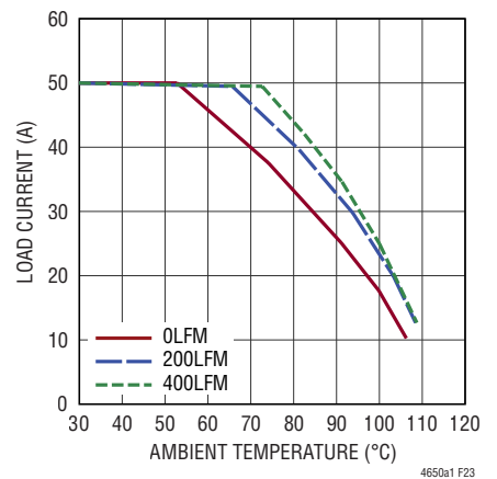
Figure 23. 12V to 1.8V Derating Curve, No Heat Sink
