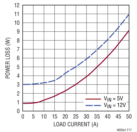
Figure 17. 3.3V OUT Power Loss Curve
