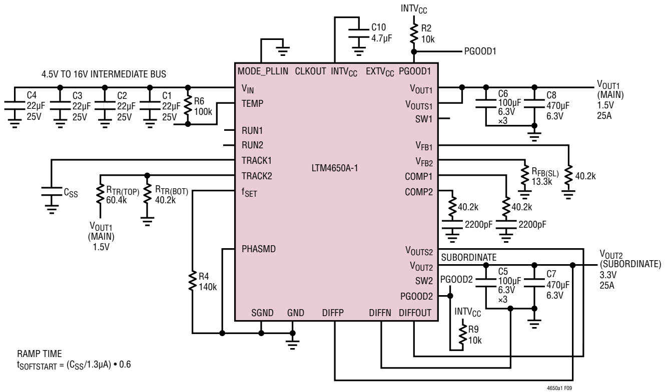
Figure 9. Example of Output Tracking Application Circuit
