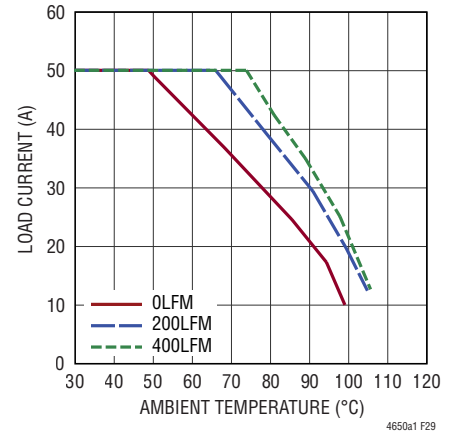
Figure 29. 12V to 3.3V Derating Curve, BGA Heat Sink
