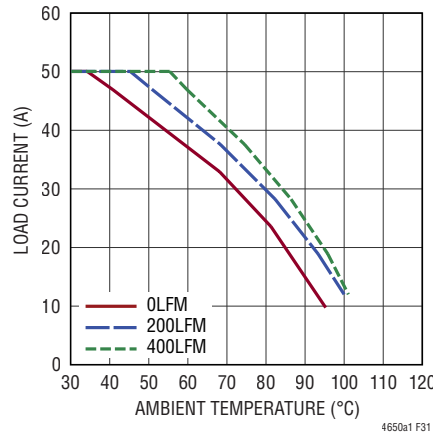
Figure 31. 12V to 5V Derating Curve, No Heat Sink
