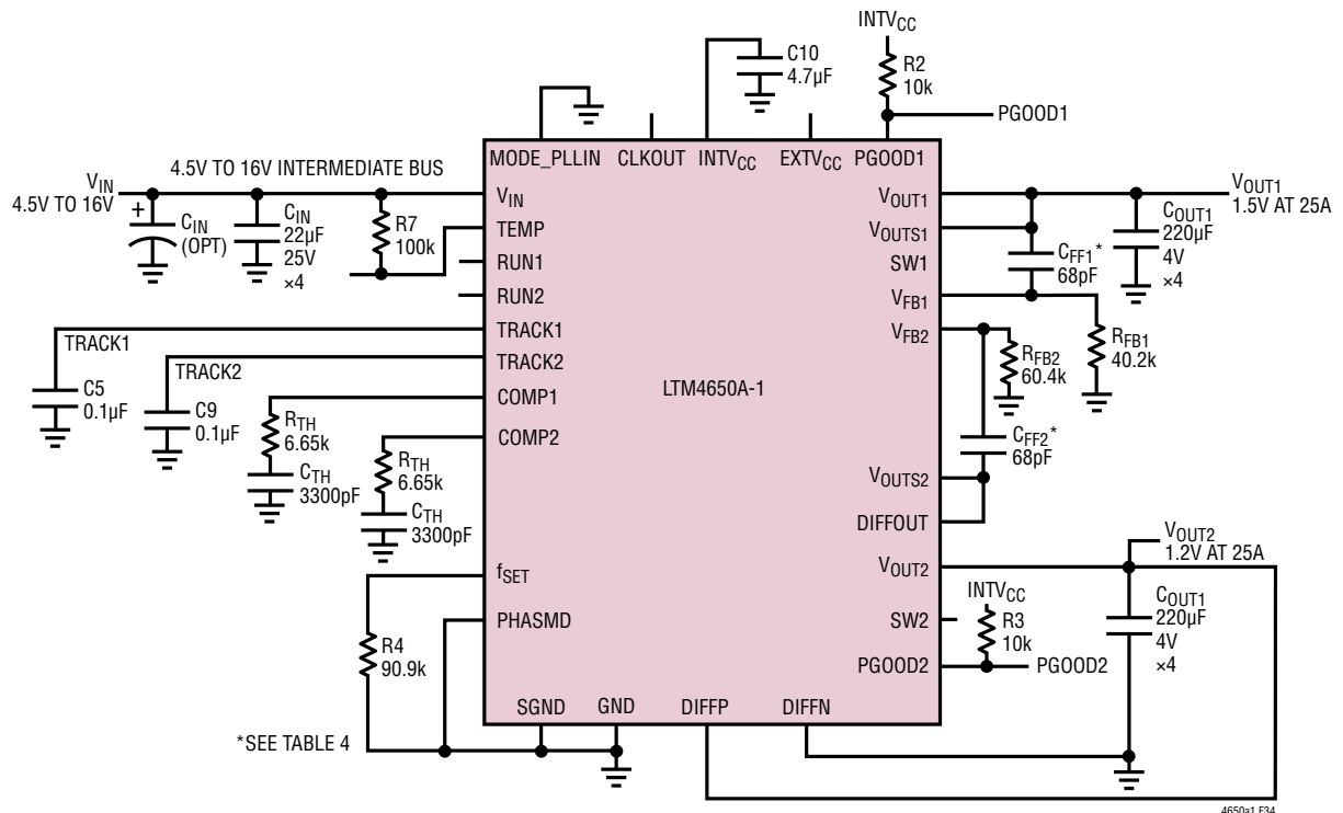
Figure 34. Typical 4.5V IN to 16V IN , 1.5V and 1.2V at 25A Outputs
