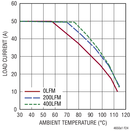
Figure 24. 5V to 1.8V Derating Curve, No Heat Sink
