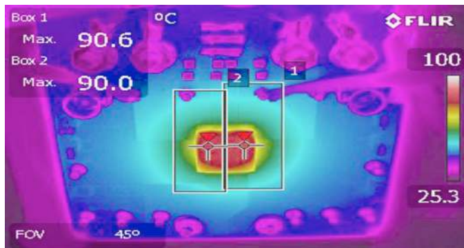
Figure 13. Thermal Image 12V to 1.0V, 50A with No Airflow without Heat Sink
