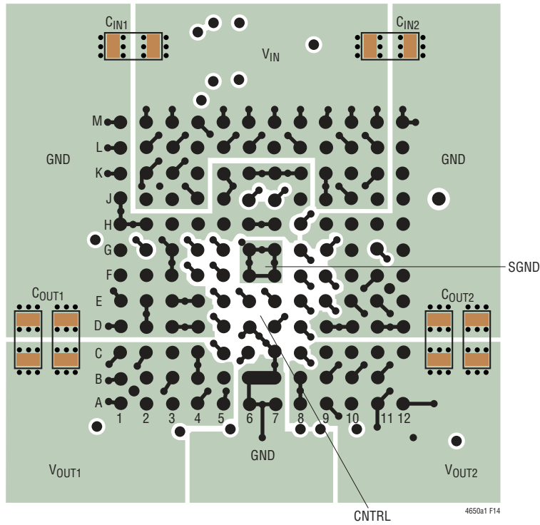
Figure 33. Recommended PCB Layout
