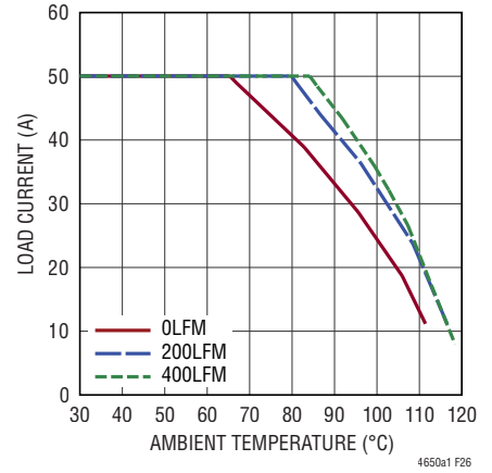
Figure 26. 5V to 1.8V Derating Curve, BGA Heat Sink
