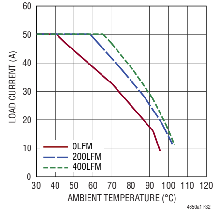
Figure 32. 12V to 5V Derating Curve, BGA Heat Sink
