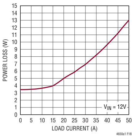
Figure 18. 5V OUT Power Loss Curve
