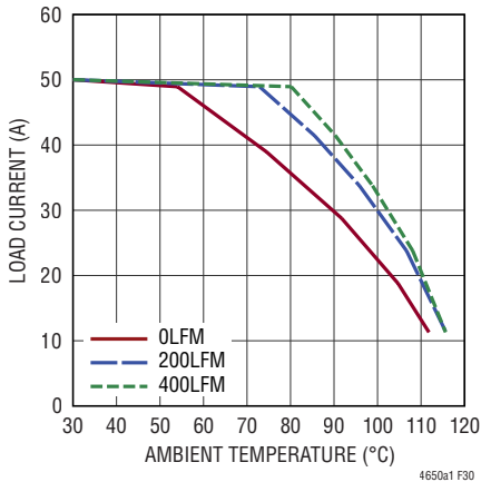
Figure 30. 5V to 3.3V Derating Curve, BGA Heat Sink
