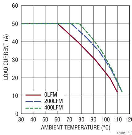
Figure 19. 12V to 1V Derating Curve, No Heat Sink
