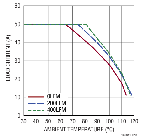
Figure 20. 5V to 1V Derating Curve, No Heat Sink
