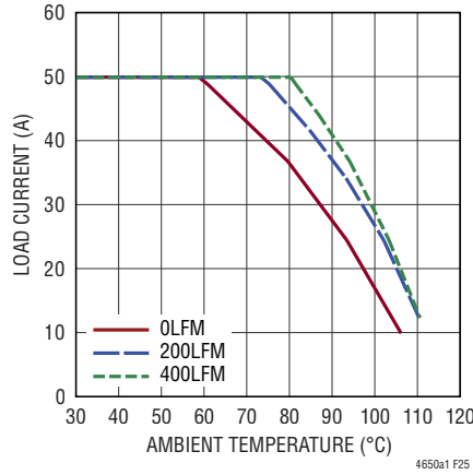
Figure 25. 12V to 1.8V Derating Curve, BGA Heat Sink
