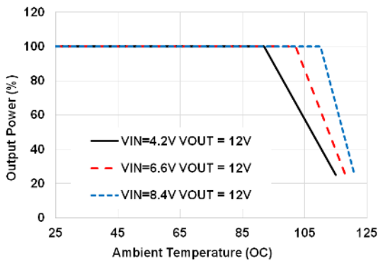
Power Derating V_{IN} = 4.2V , 6.6V , and 8.4V , V_{OUT} = 12V
