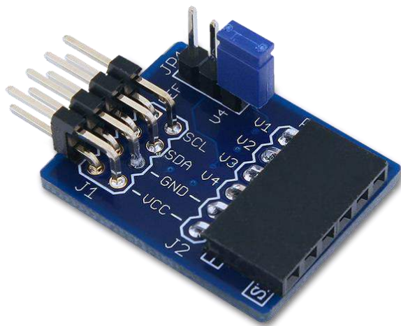
The PmodAD2.
