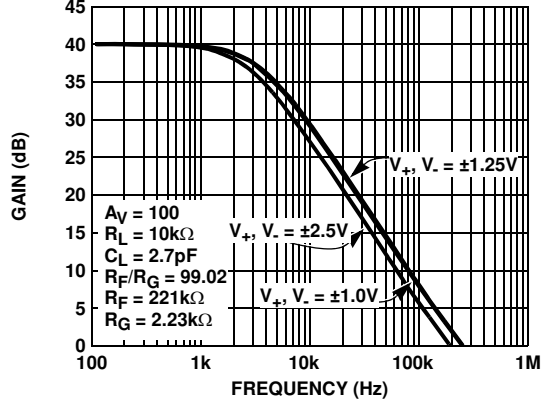
FIGURE 4. ISL28276, ISL28476 FREQUENCY RESPONSE vs SUPPLY VOLTAGE
