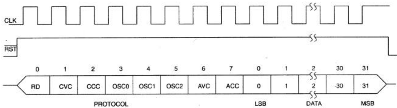
Figure 3. DATA TRANSFER
