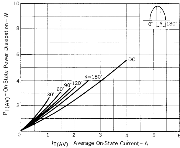
Fig. 9 P_T(I_{T(AV)}) CHARACTERISTIC
