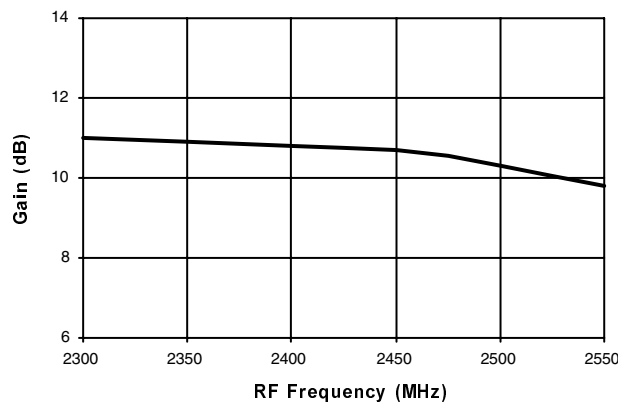
Figure 3. Conversion Gain versus RF Frequency, V_{CC} = 5.0\text{ V} , LO = 0\text{ dBm} , RF_{IN} = -20\text{ dBm} , IF = 200 MHz
