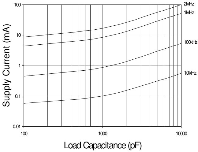
Fig. 19 Supply Current vs. Capacitive Load V_{SUPPLY} = 15V
