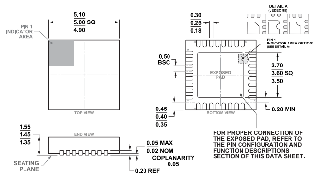
Figure 30. 32-Lead Lead Frame Chip Scale Package [LFCSP] 5 mm x 5 mm Body, Thick Quad (CP-32-17) Dimensions shown in millimeters
