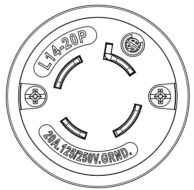
FACE VIEW
