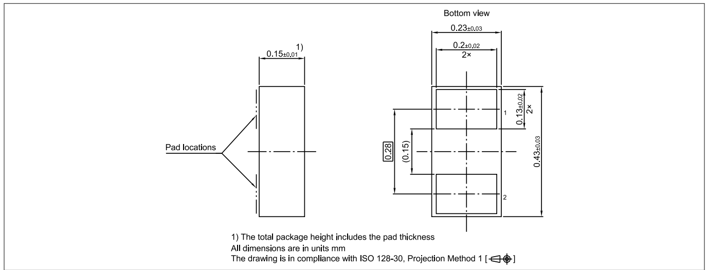
Figure 12 Package outline
