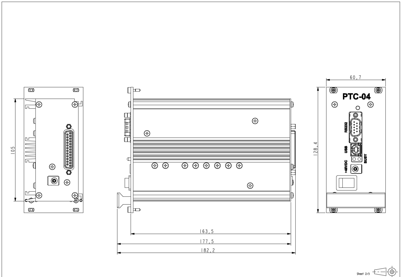
Figure 21-1: Mechanical Outlines
