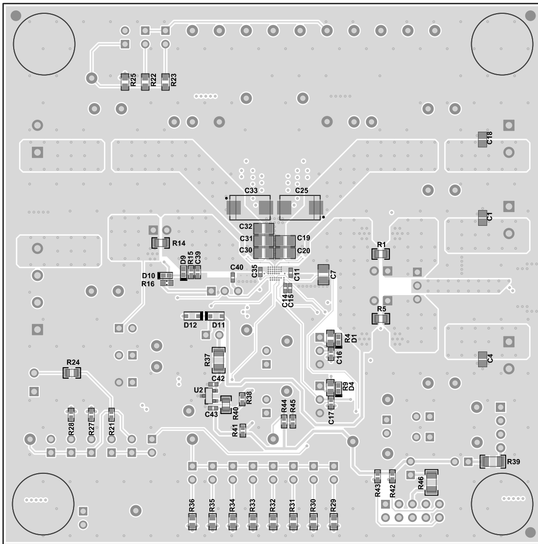
Figure 4-6. BMS027A Bottom Layer and Overlay
