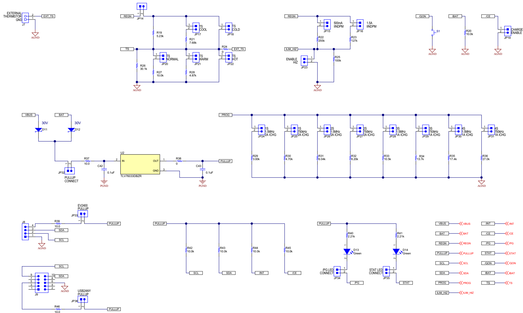
Figure 4-2. BQ25790EVM Schematic Page 2
