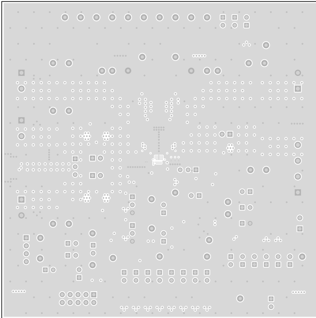
Figure 4-4. BMS027A Signal Layer 1
