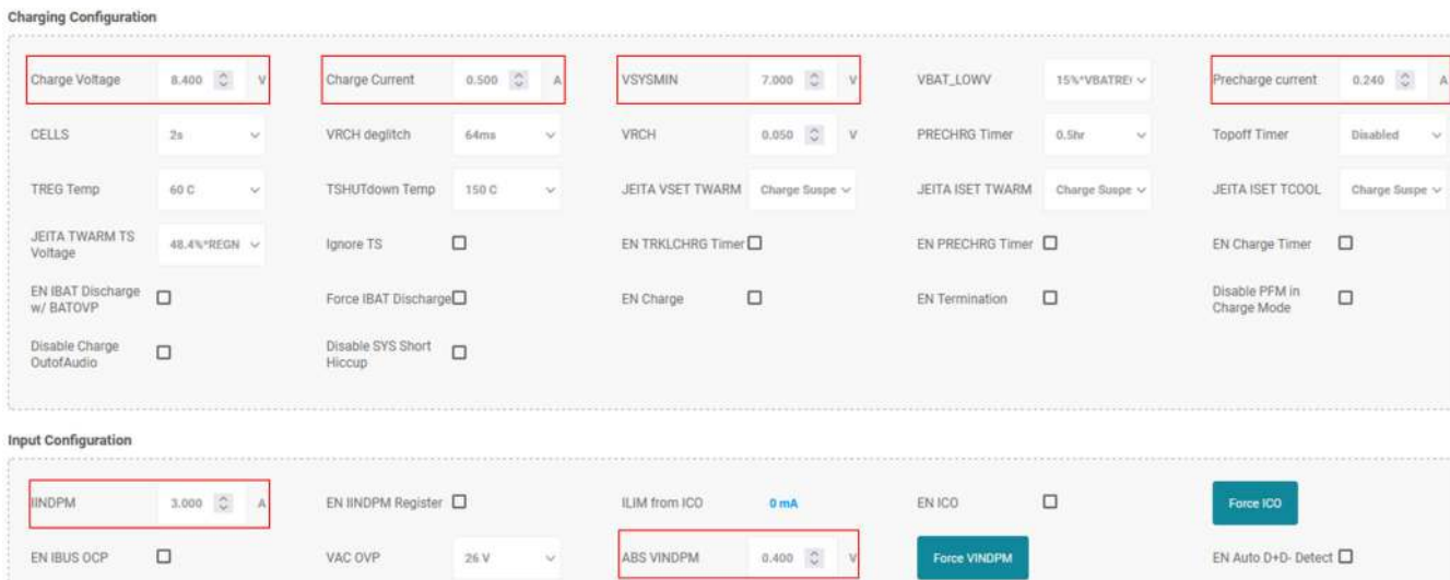
Figure 2-7. Charger Configuration
