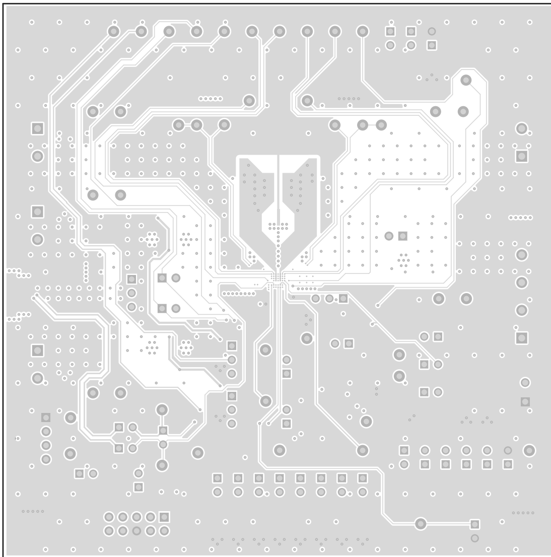
Figure 4-5. BMS027A Signal Layer 2
