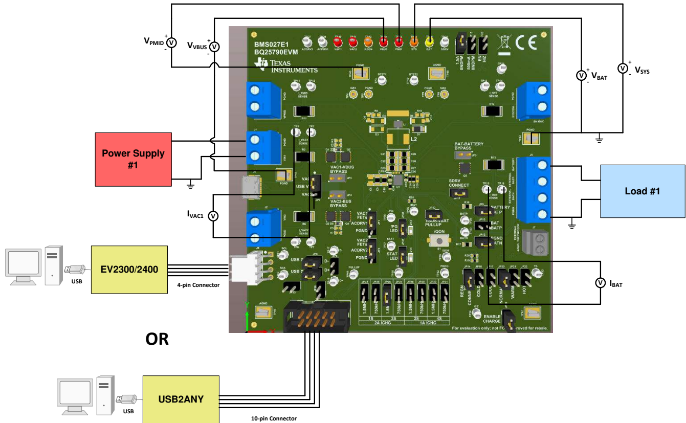
Figure 2-1. Equipment Test Setup for BMS027A
