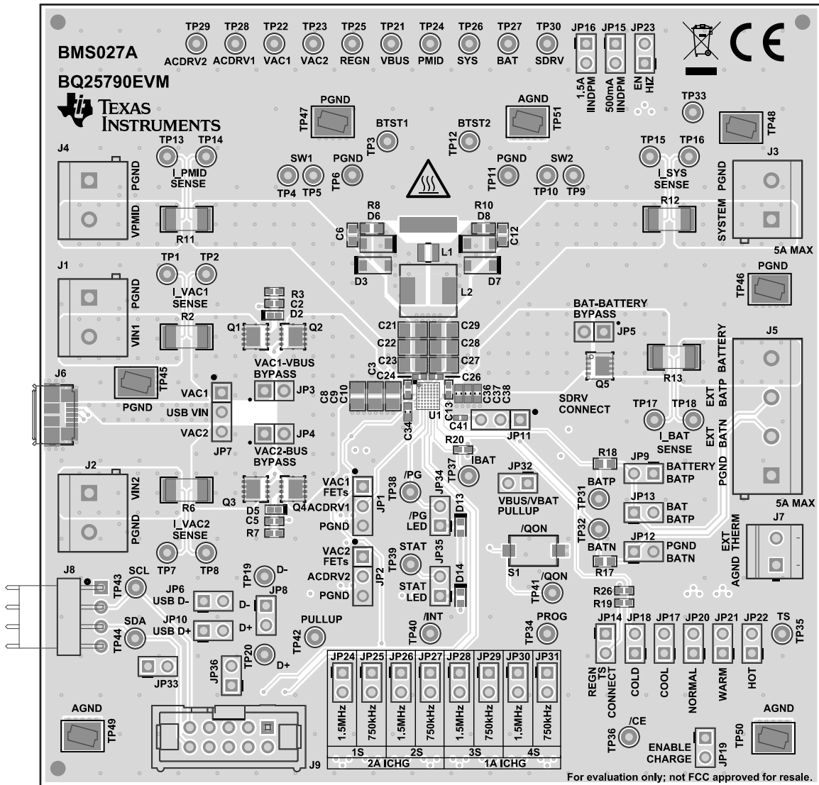
Figure 4-3. BMS027A Top Layer and Overlay
