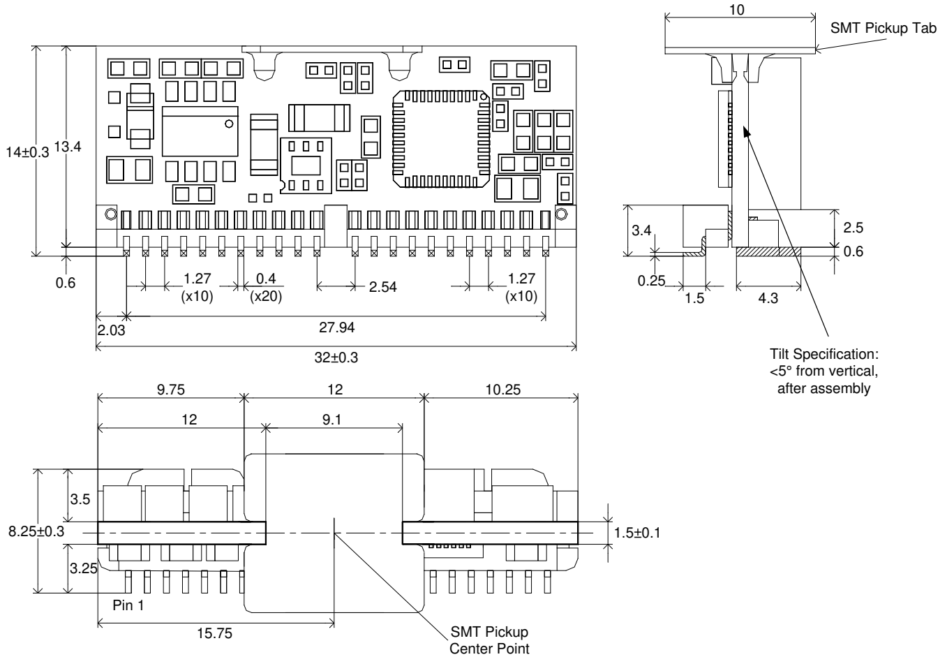
Figure 57. Mechanical Drawing
