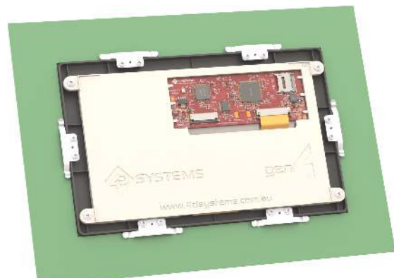
Gen4-uLCD-70DT secured to the 7.0" Bezel, and Bezel secured to the Panel/Enclosure using the supplied large spring clips and screws
