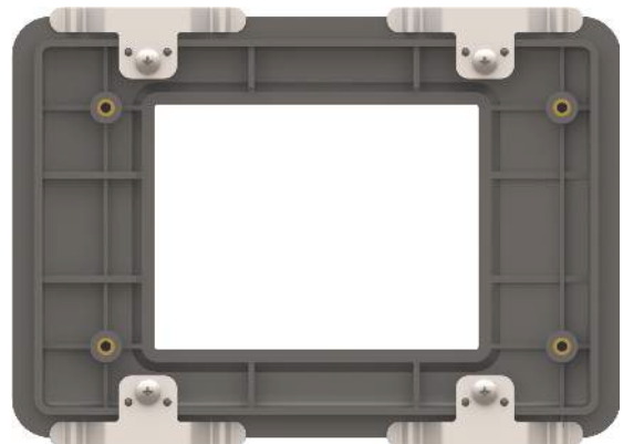
Bare 2.4" Bezel with clips attached - Back
