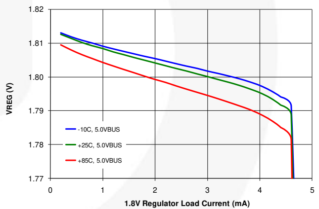
Figure 20. V_{REG} 1.8 V Output Regulation
