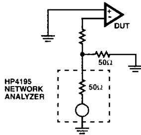
FIGURE 1. TEST CIRCUIT FOR TRANSMIMPEDANCE MEASUREMENTS
