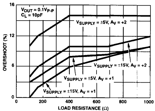
FIGURE 15. SMALL SIGNAL OVERSHOOT vs LOAD RESISTANCE
