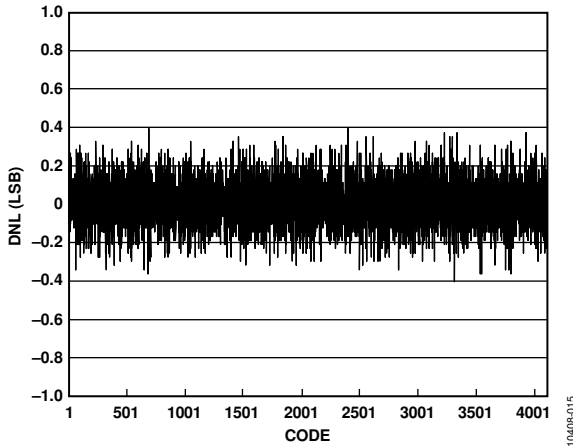
Figure 15. ADC DNL
