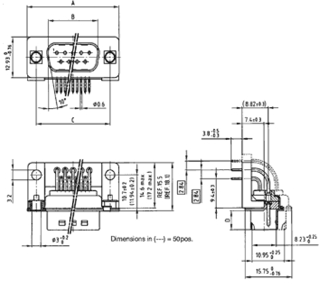
Plug connector
