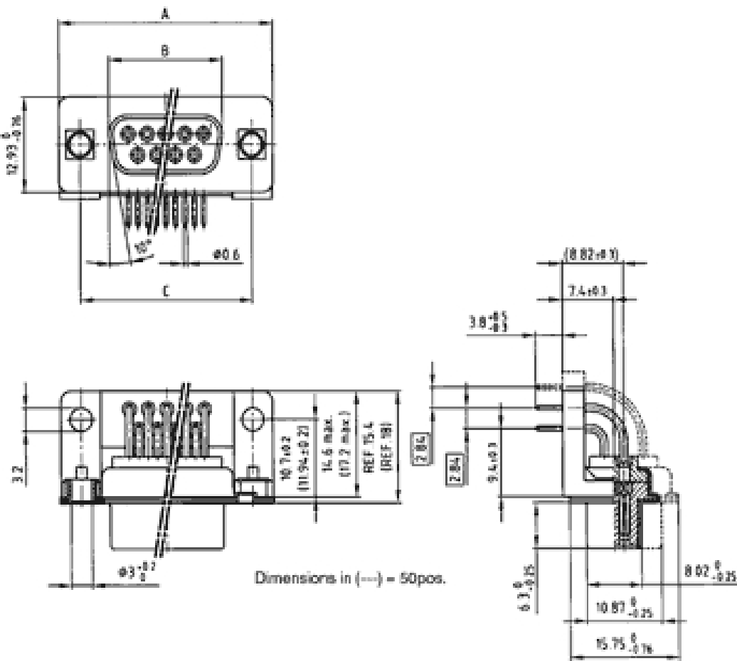
Socket connector
