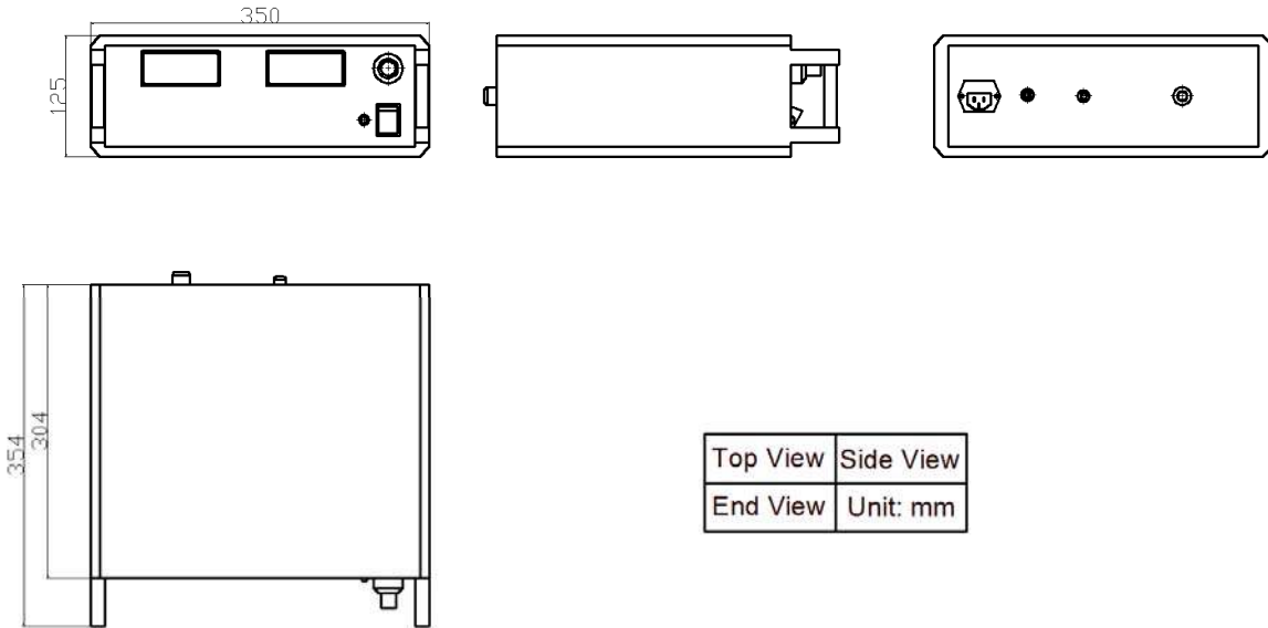
Figure 7. Dimensions for AHVAC60KVR5MABT
