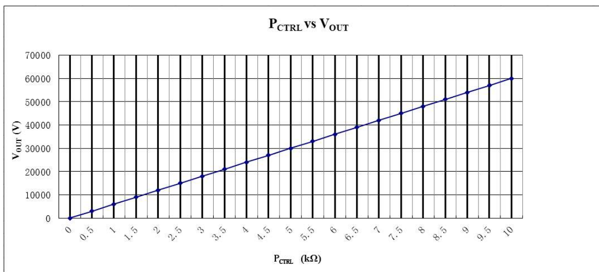
Figure 4. P_CTRL vs. V_OUT
