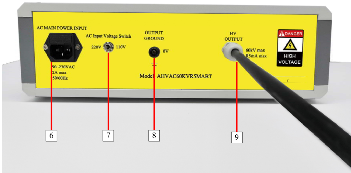
Figure 3. Front Panel
