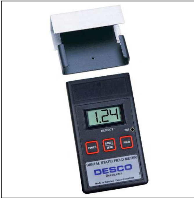
Figure 3. Installing the 19441 Conductive Plate
