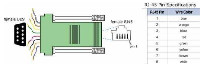
Figure 11. Female RS-485/422 Adapter and pin specifications
