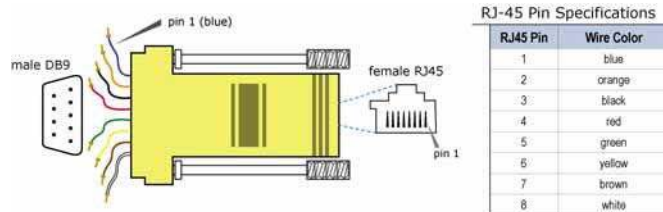
Figure 10. Male RS-485/422 Adapter and pin specifications
