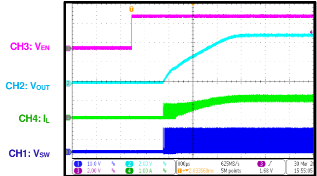
Start-Up through EN I_{OUT} = 1A
