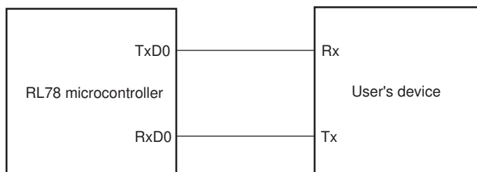
UART mode connection diagram
