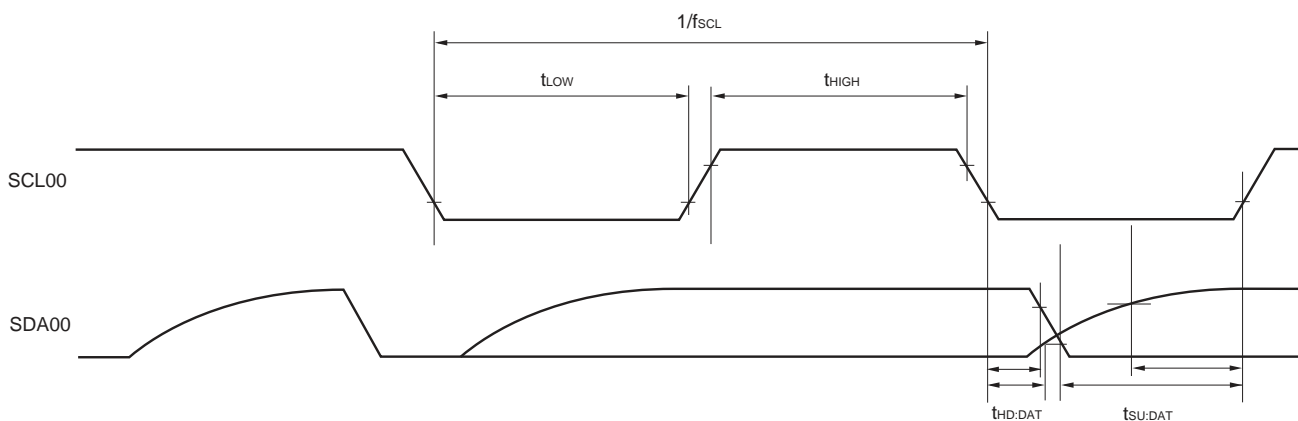
Simplified I 2 C mode serial transfer timing
