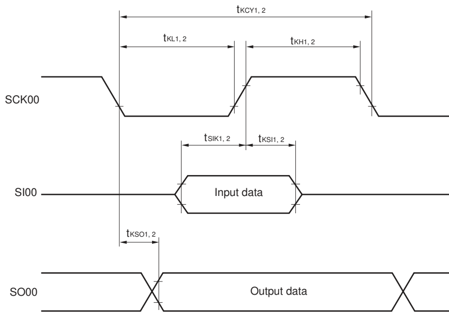
Simplified SPI (CSI) mode serial transfer timing (When DAP0n = 0 and CKP0n = 0, or DAP0n = 1 and CKP0n = 1.)
