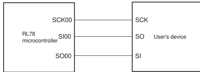
Simplified SPI (CSI) mode connection diagram
