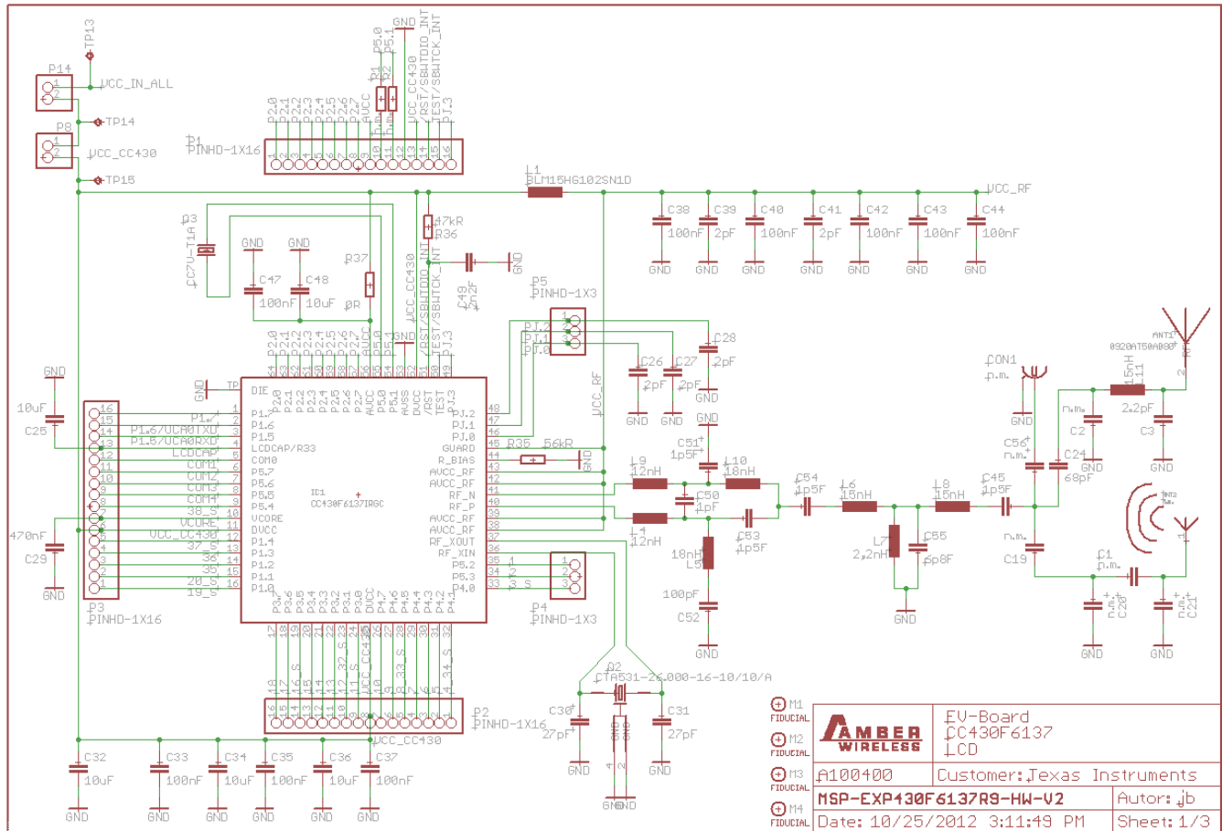
Figure 7. MSP-EXP430F6137Rx Base Board Schematic – Page 1
