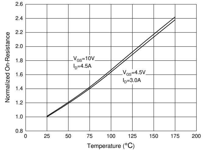
Fig. 6 - R_{DS(ON)} - \text{Temperature}
