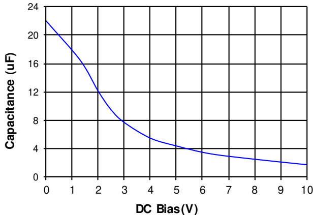
Figure 40. C EFF for 22 µF, 0603, X5R, 10 V-Rated Capacitor (TDK C1608X5R1A226M080AC)
