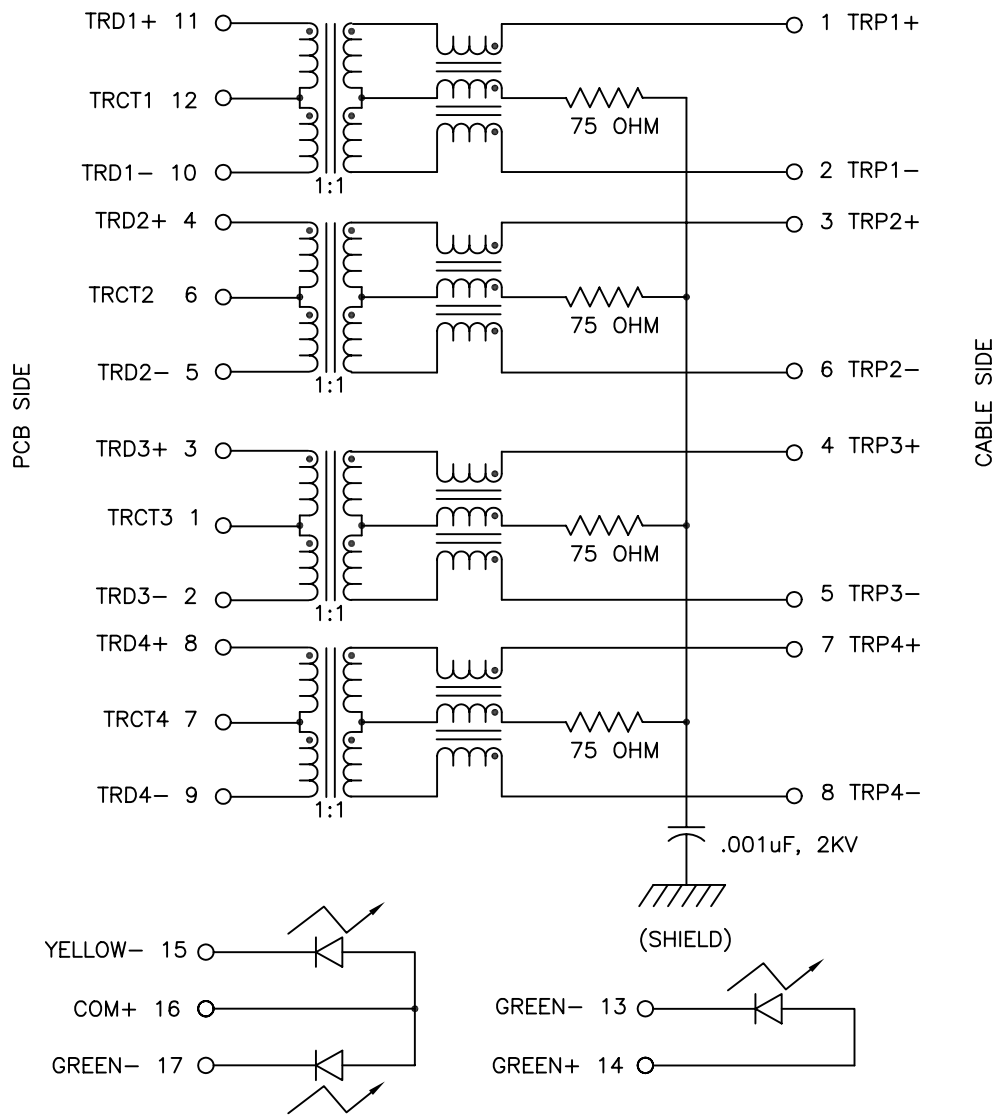
SCHMATIC
