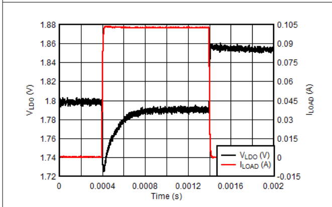
Figure 8-18. LDO Load Transient - VLDO = 1.8V
