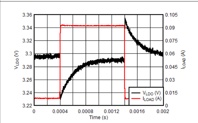
Figure 8-19. LDO Load Transient - VLDO = 3.3V
