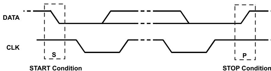
Figure 7-9. START and STOP Condition
