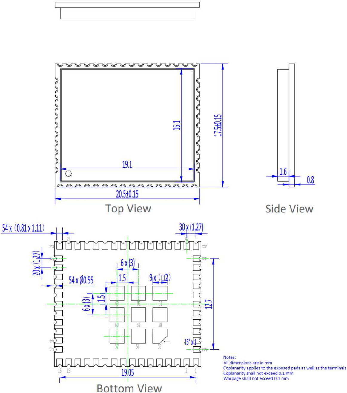
Figure 5-1: Mechanical Drawing
