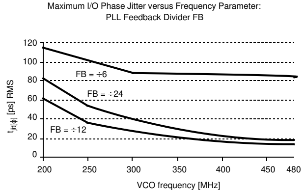
Figure 10. MPC9773 I/O Jitter
