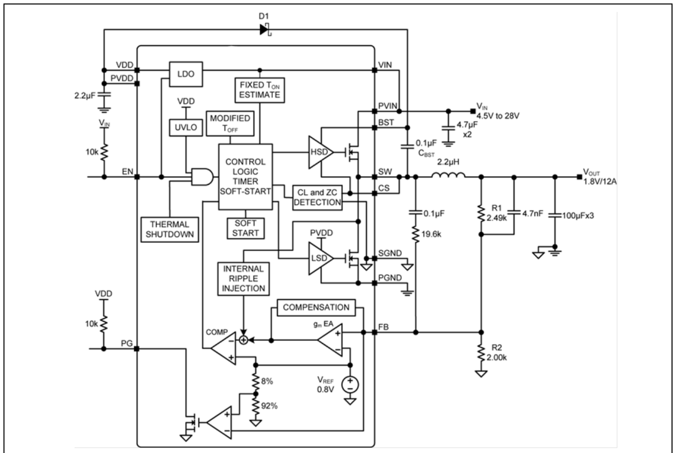
Figure 2.1 Functional Diagram
