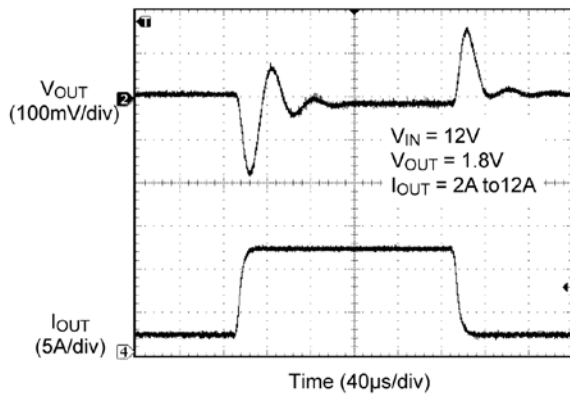
Transient Response
