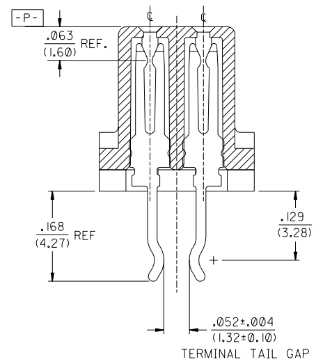
SECTION "Z-Z" SCALE 8:1
