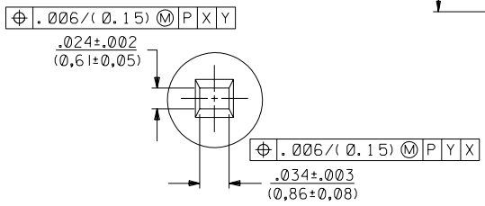
PIN WINDOW DETAIL
