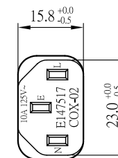
CONNECTOR: COX-02
