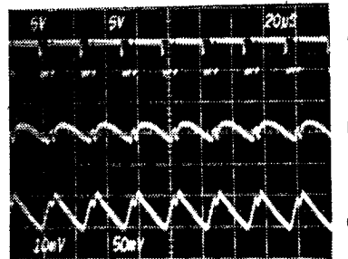
MAX741U SWITCHING WAVEFORMS – BURST-MODE
