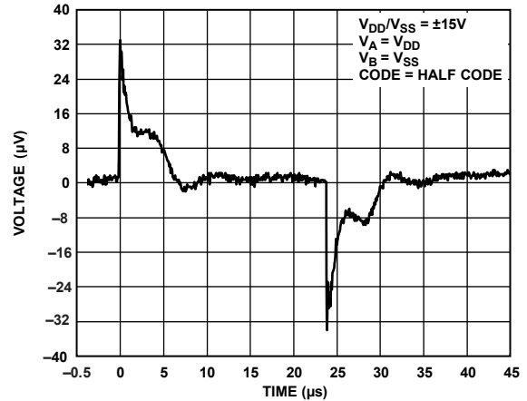
Figure 53. Digital Feedthrough
