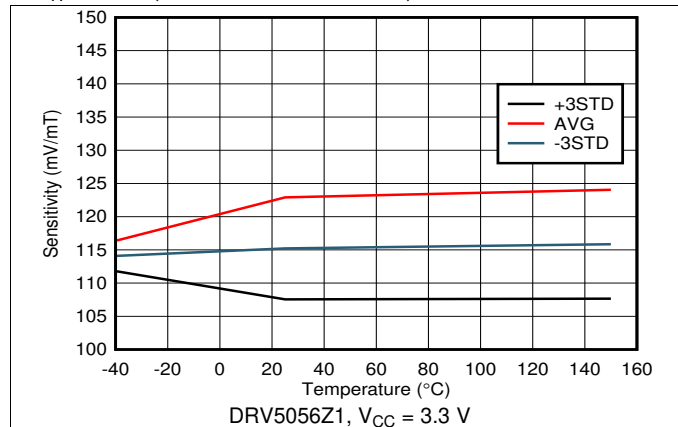
Figure 19. Sensitivity vs Temperature
