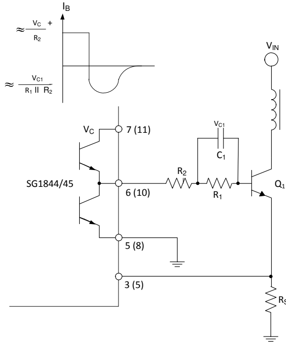
Figure 18 · Bipolar Transistor Drive
