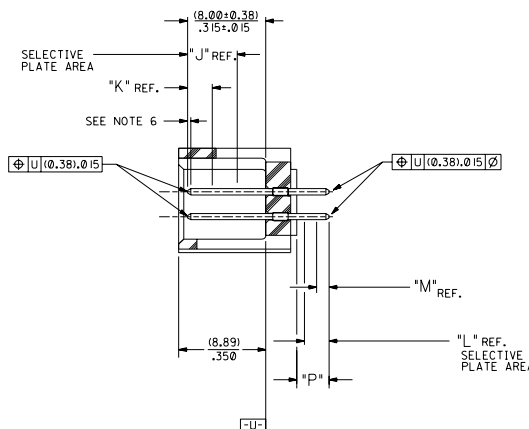
SECTION J-J
