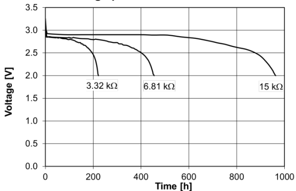
Discharge performance at 23°C
