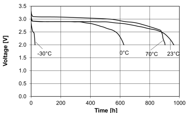
Temperature performance Load 15kΩ
