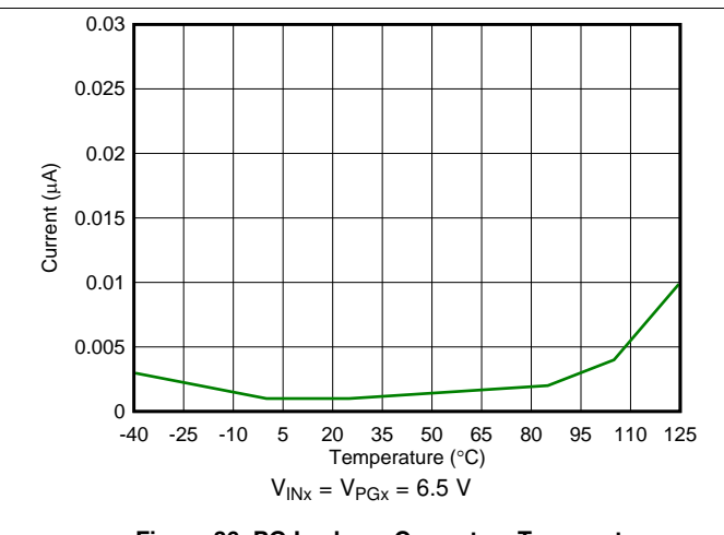
Figure 36. PG Leakage Current vs Temperature
