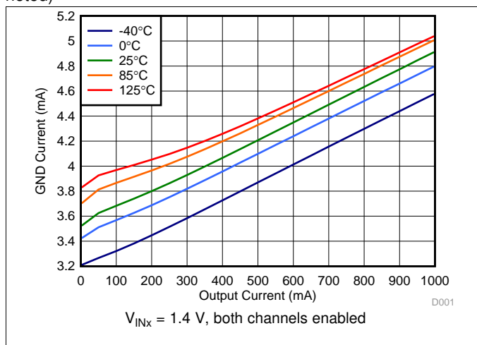
Figure 31. Ground Current vs Output Current
