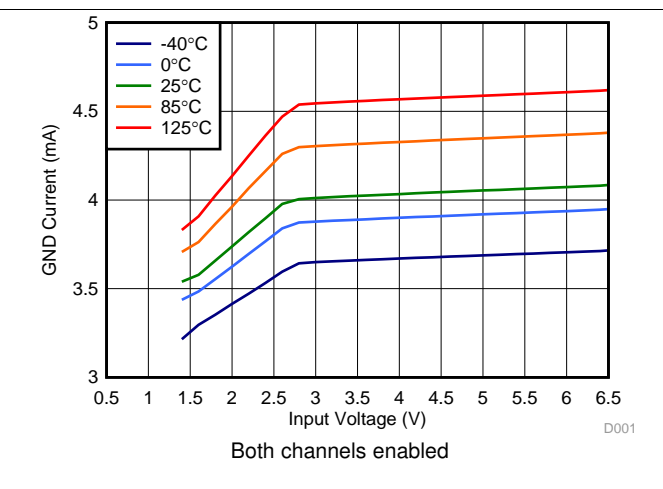
Figure 32. Ground Current vs Input Voltage
