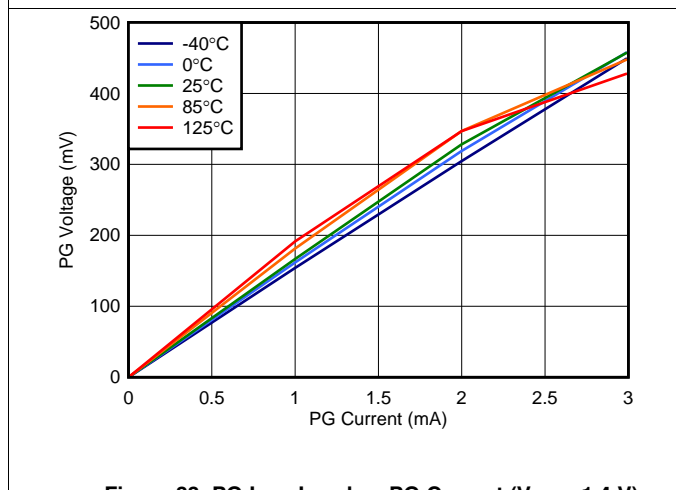
Figure 33. PG Low Level vs PG Current ( V_{\text{INX}} = 1.4\text{ V} )
