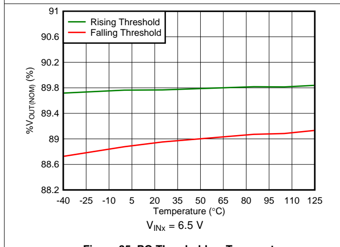
Figure 35. PG Threshold vs Temperature
