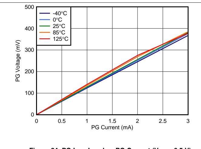
Figure 34. PG Low Level vs PG Current ( V_{\text{INX}} = 6.5\text{ V} )
