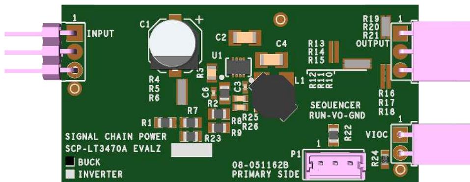
Figure 1. SCP-LT3470A-BEVALZ Board
