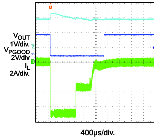
Over-Voltage Protection
