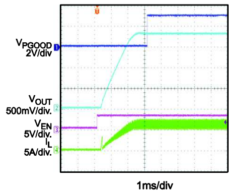
Power-Up through EN I_{OUT} = 6A , Pulse Skip
