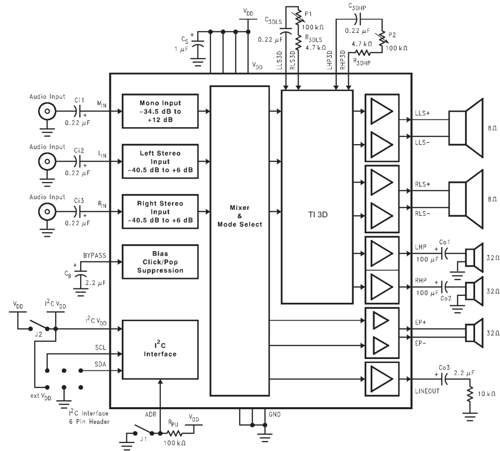
Figure 55. Reference Design Board Schematic
