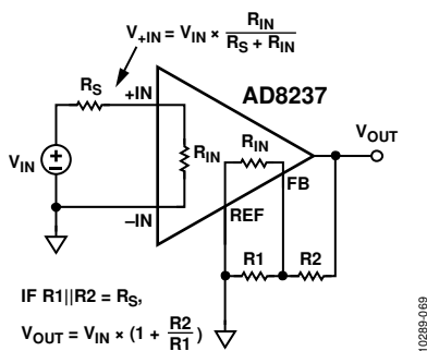
Figure 67. Cancelling Input Impedance Errors
