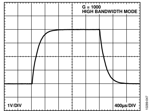
Figure 45. Large Signal Pulse Response, High Bandwidth Mode, G = 1000, R_L = 10 \text{ k}\Omega, C_L = 10 \text{ pF}
