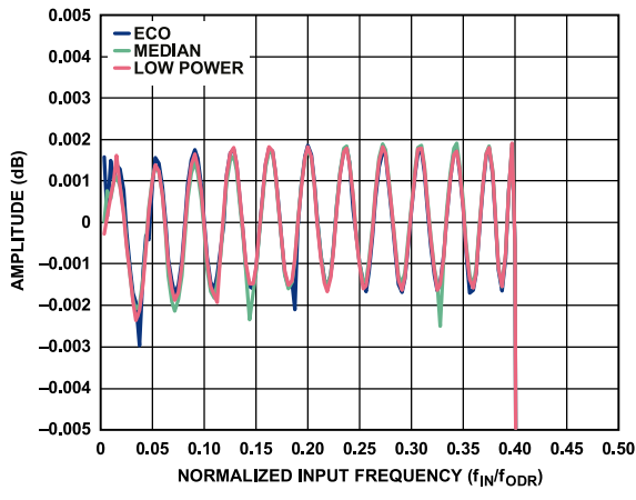
Figure 59. Wideband Filter Ripple
