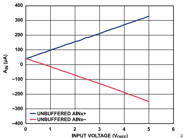
Figure 85. Analog Input Current ( I_{AIN} ) vs. Input Voltage, Analog Input Precharge Buffer Off, V_{CM} = 2.5 V, f_{MOD} = 8.192 MHz
