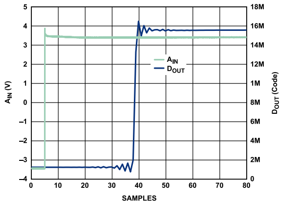
Figure 58. Step Response, Wideband Filter
