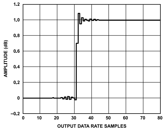
Figure 92. Wideband Filter Step Response
