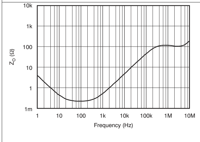
Figure 9. Open-Loop Output Impedance vs Frequency
